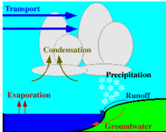
Figure 1 – Hydrological cycle 1
