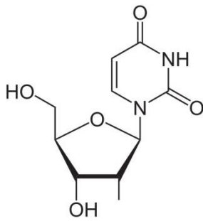
2'-uridylyl-
