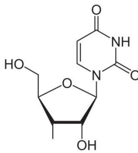
3'-uridylyl-
