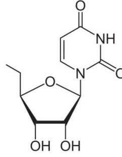
5'-uridylyl-
